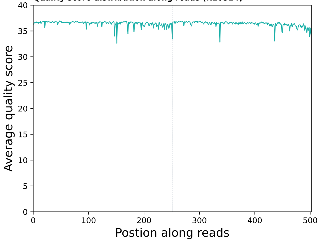
Quality score distribution along reads (R10324)
